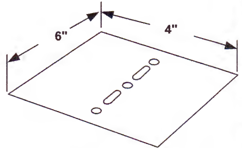
18 GA GALV. 4 X 6 BEARING PLATE
