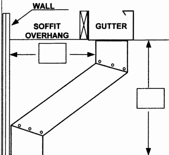
ONE PIECE "A" ELBOW RETURN OFFSET
