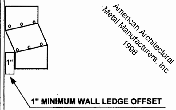
ONE PIECE "A" ELBOW RETURN OFFSET
